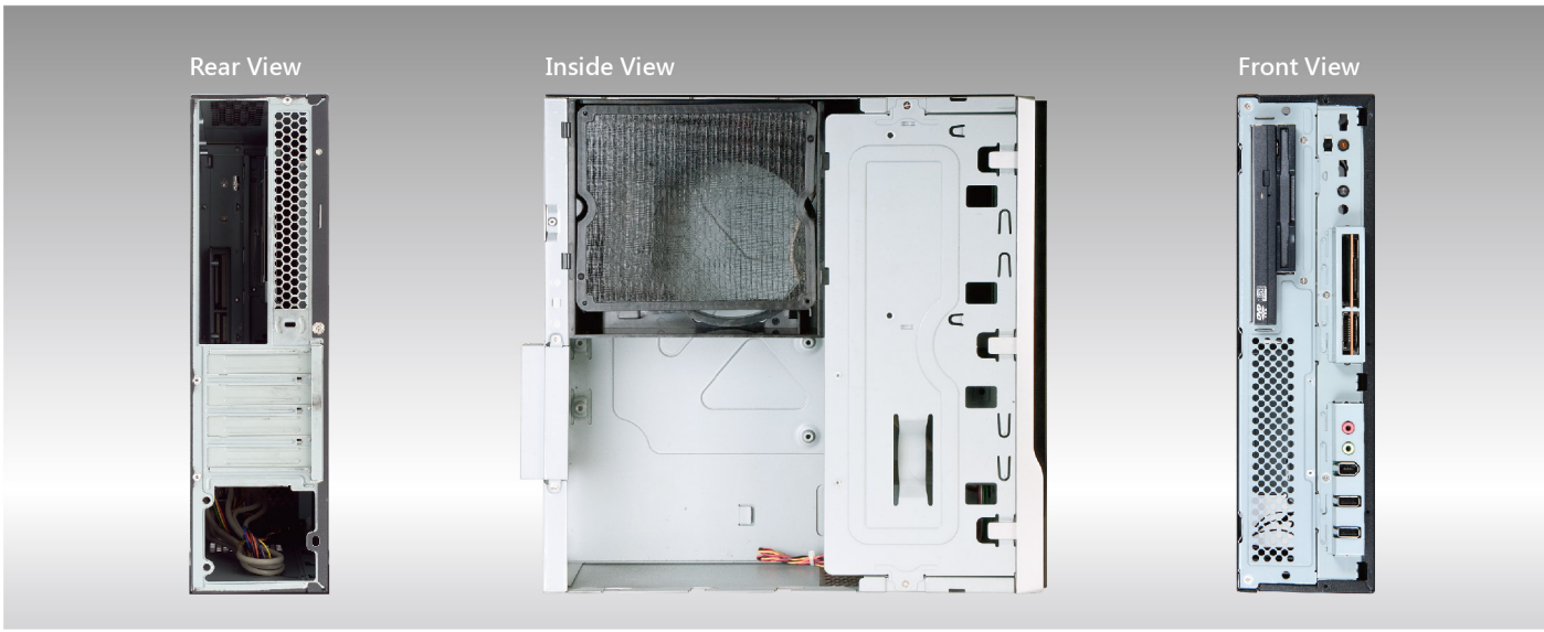
Optional card reader Removable drive cage Slim ODD, Slim FDD, internal 3.5" bays Side (bottom) 1 x bottom 60 mm fan Optional TFX PSU
